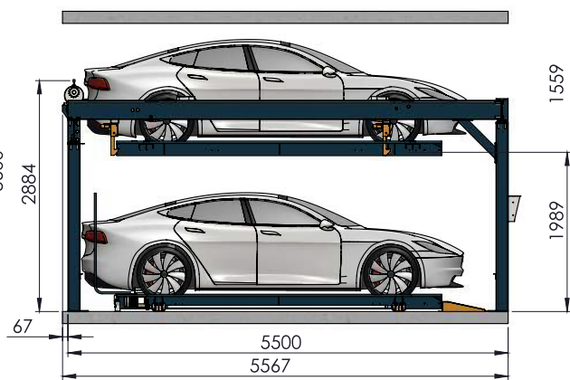
Puzzle 5 cars sedan SIDE-VIEW
