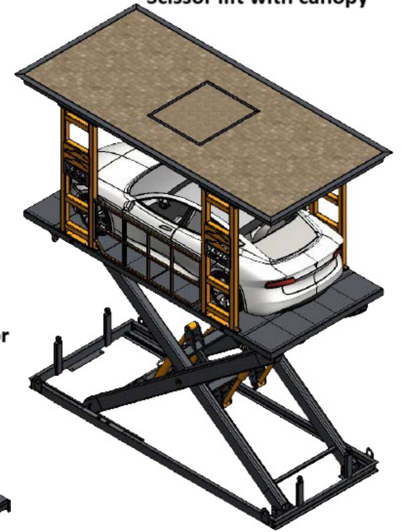
Scissor lift with canopy
