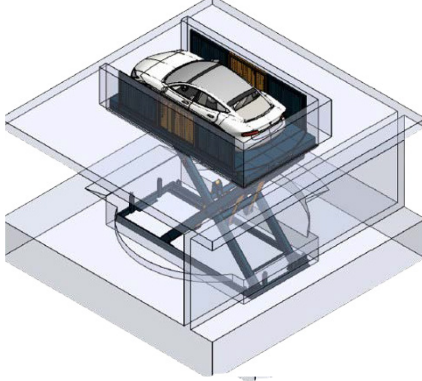
Scissor lift with turn table
