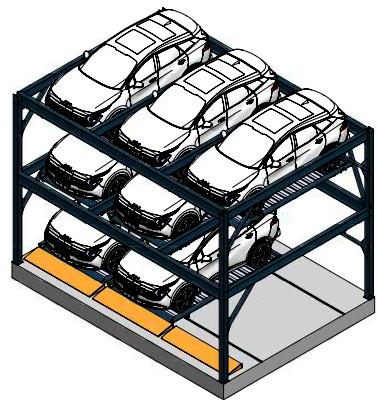
Puzzle 7 cars (3 bays / 3 levels)
