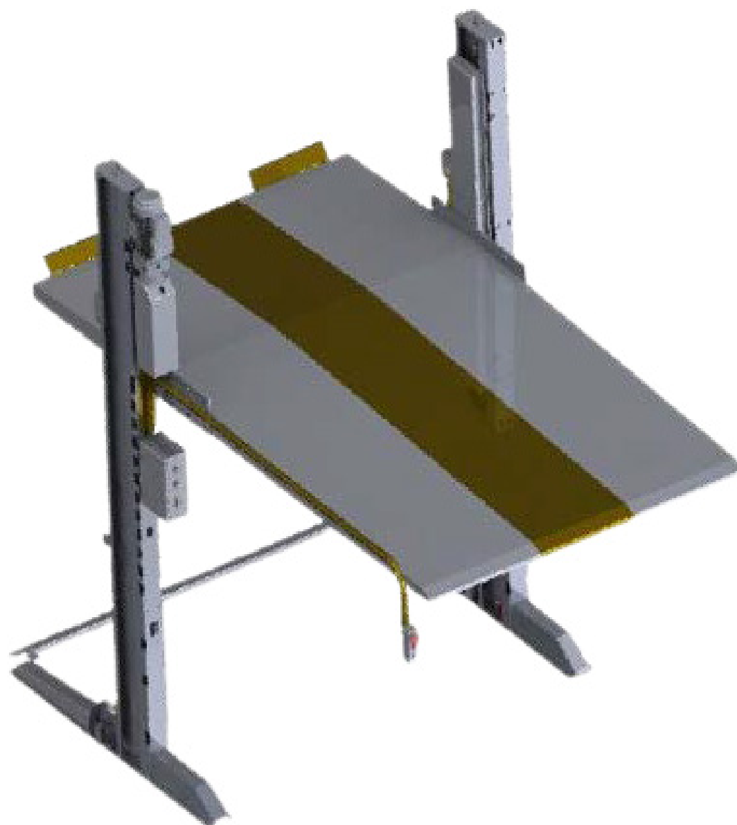
Two Post Parking Lift – sport cars special edition (The lowest ground clearance – up to 8 cm)
